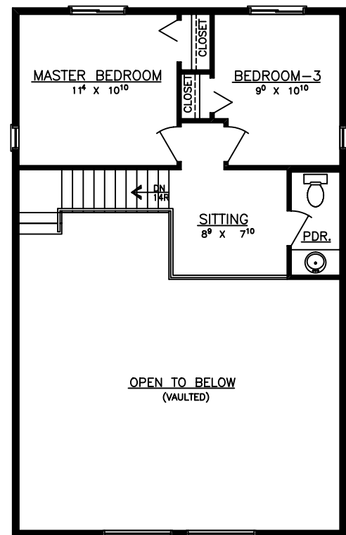
SECOND FLOOR AREA = 375 S.F.
