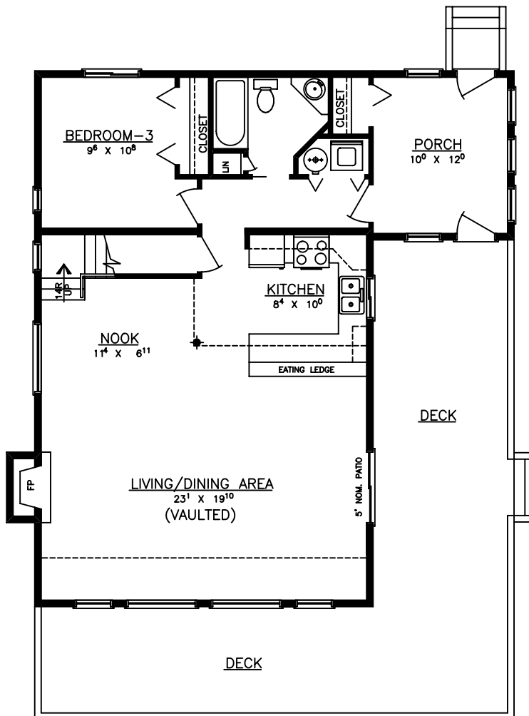
MAIN FLOOR AREA = 1032 S.F.
